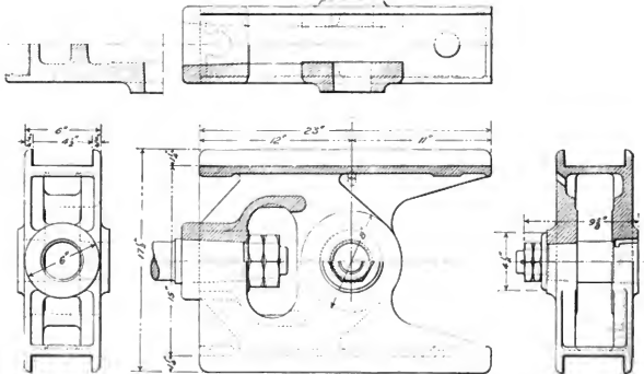
Figs. 1087-1091. Alligator Crosshead. Baldwin Locomotive Works.
